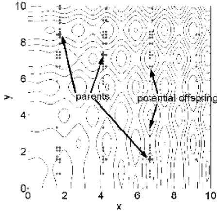
Figure 5.12 Three parents and potential offspring from three-point crossover in a binary GA.
